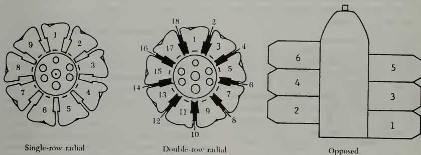
FIGURE 1-15. Numbering of engine cylinders.
